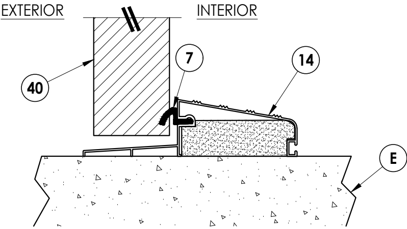
2 6 VERTICAL CROSS SECTION Outswing Threshold
