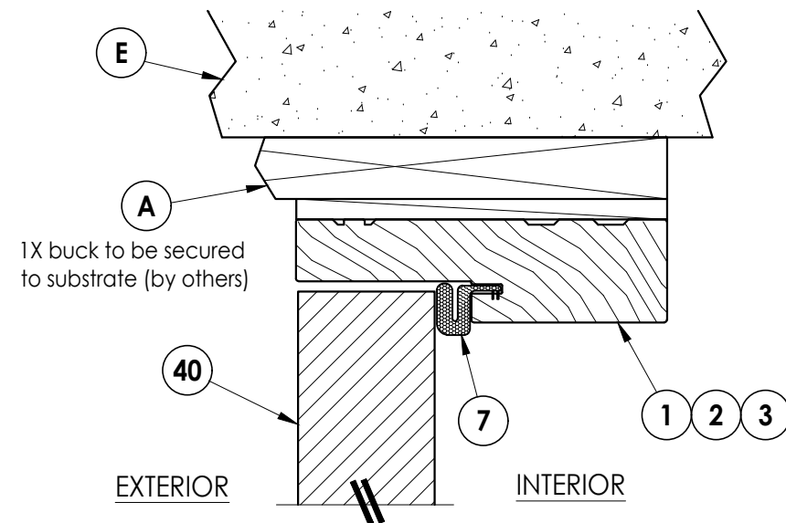
1 VERTICAL CROSS SECTION 4 Outswing shown (Inswing similar)
