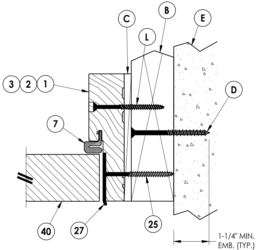
2 HORIZONTAL CROSS SECTION 3 Outswing shown (Inswing similar)
